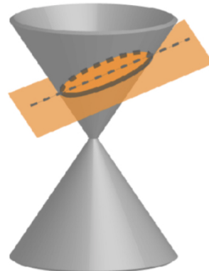
Ellipse
