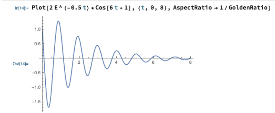
Figure 6: A damped oscillator, plotted using Mathematica function Plot.
